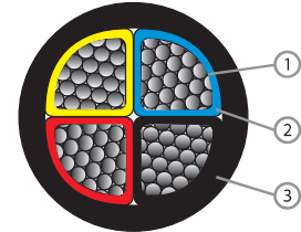
Component 1-Aluminium Wire 2-PVC Compound 3-PVC Compound
