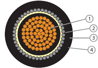
Component 1. Copper Wire 2. PVC Compound 3. Aluminium Wire Armoured 4. PVC Compound
