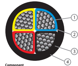
Component 1- Aluminium Wire 2- Cross-linked Polyethylene Compound 3- PVC Compound
