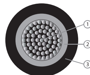
Component 1. Aluminum Wire 2. Cross-linked Polyethylene Compound 3. PVC Compound
