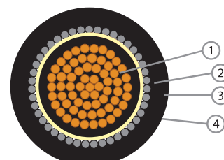
Component 1. Copper Wire 2. Cross-linked Polyethylene Compound 3. Aluminium Wire Armoured 4. PVC Compound
