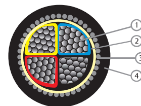
Component 1. Aluminium Wire 2. PVC Compound 3. Galvanised Steel Wire Armoured 4. PVC Compound
