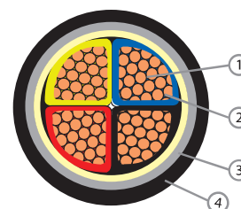
Component 1-Copper Wire 2-PVC Compound 3-Galvanised Steel Tape Armoured 4-PVC Compound
