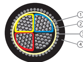
Component 1. Aluminium Wire 2. Cross-linked Polyethylene Compound 3. Galvanised Steel Wire Armoured 4. PVC Compound
